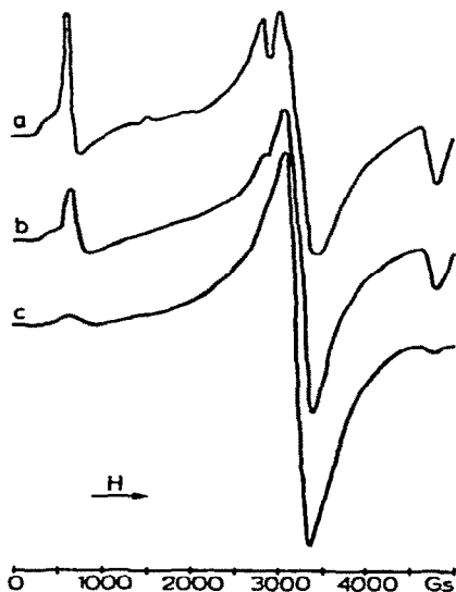
Fig. 4. EPR spectrum of the reaction mixture \text{FeCl}_3 + \text{Mg} + \text{THF} ; (a) without mixing of substrates; (b) slow mixing of substrates; (c) fast mixing of substrates.
